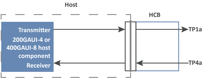
Figure 120E-5--Host 200AUI-4 or 400GAUI-8 C2M compliance points
