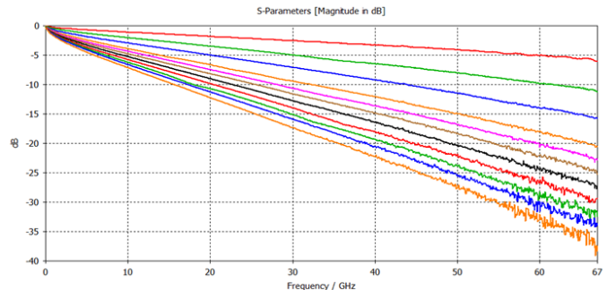
92 Ohms Insertion Loss
